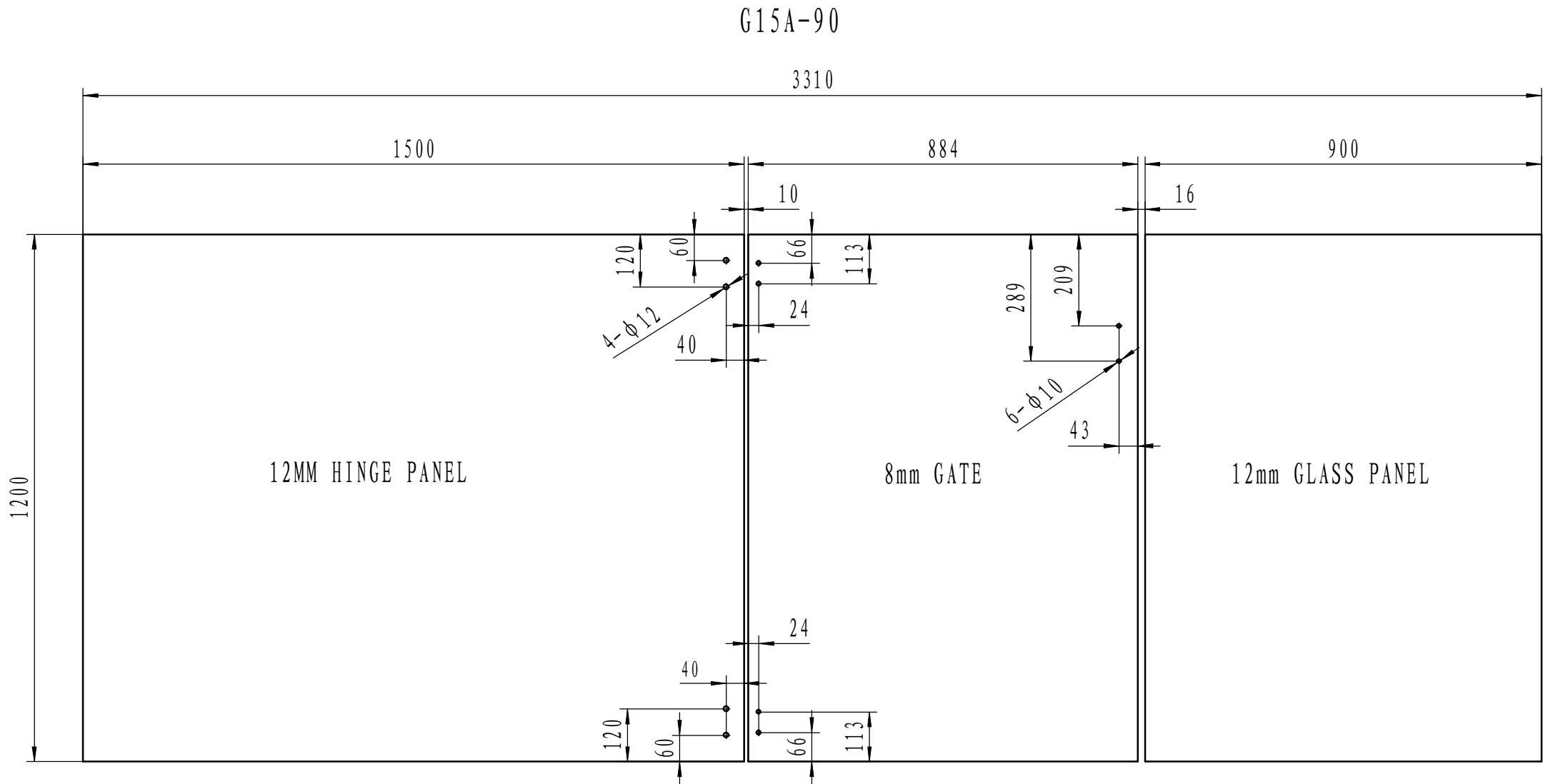
G15A-90 Tight Measurements between 3,330mm - 3,490mm
